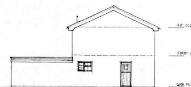
SIDE ELEVATION (NW)
